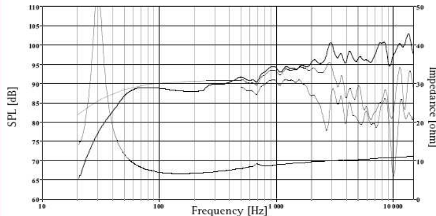
The frequency responses above show measured free field sound pressure in 0, 30, and 60 degrees angle using a 60L closed box. Input 2.83 Vrms, microphone distance 0.5m, normalized to SPL 1m. The dotted line is a calculated response in infinite baffle based on the parameters given for this specific driver. The impedance is measured in free air without baffle using a 2V sine signal.
