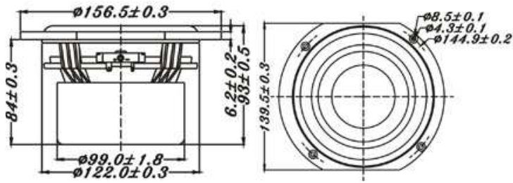
5" KEVLAR FIBER WOOFER
